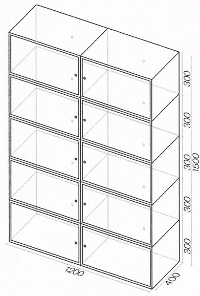
Acrylic cabinet Two to ten doors Model no. 1060/2-10
